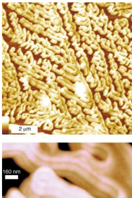
Figure 5. AFM image of rigid-rod \beta -fibril self-assemblies on graphite at low (top, vertical scale bar = 80 nm) and high magnification (bottom, 5 \mu\text{m} 2 , 3.3 mM MES, pH 5.5; for tentative structure, see 6 in Figure 1).
